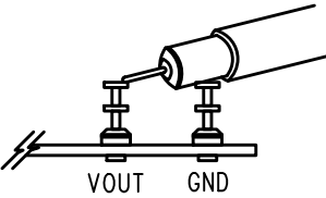
Figure 4. Measuring Output Ripple
