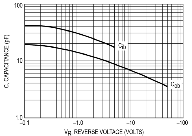
Capacitances
