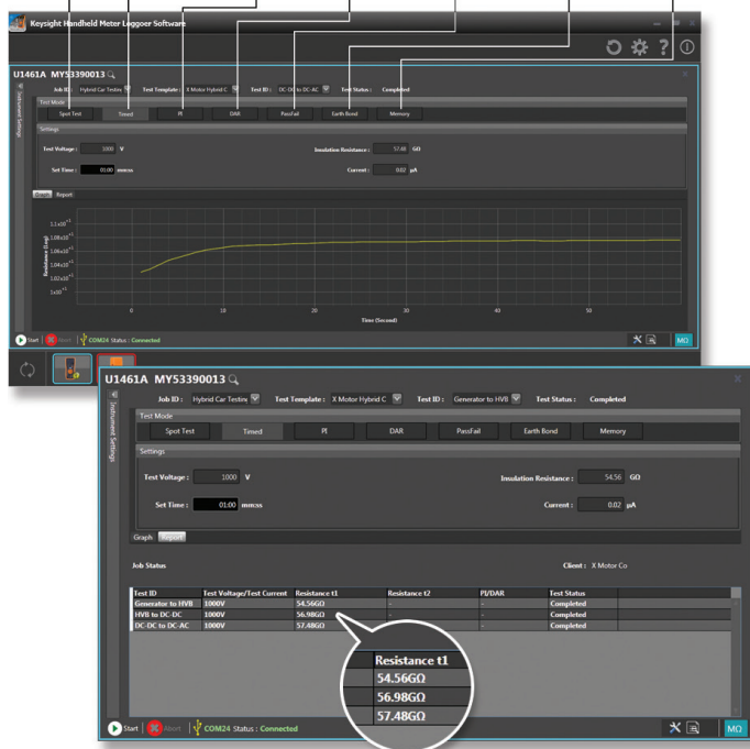
Figure 1. Keysight Handheld Logger Software Interface for Windows PC with guided operation and one button automatic report generation
