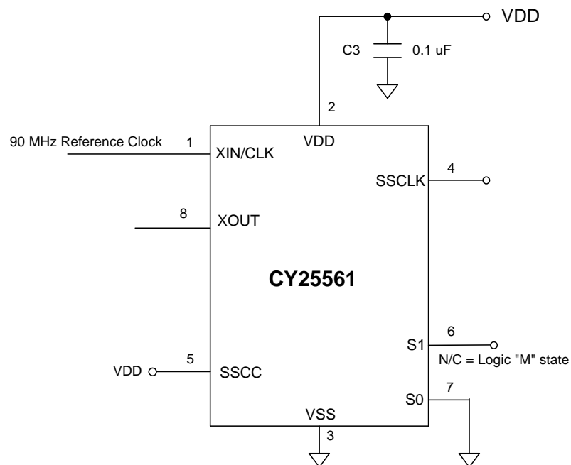
Figure 4. Application Schematic
