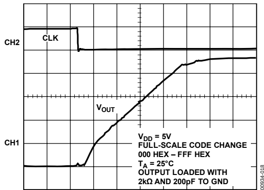
Figure 18. Full-Scale Settling Time
