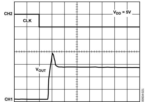
Figure 21. Exiting Power-Down (800 Hex Loaded)
