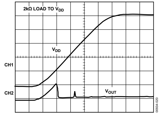
Figure 20. Power-On Reset to 0 V
