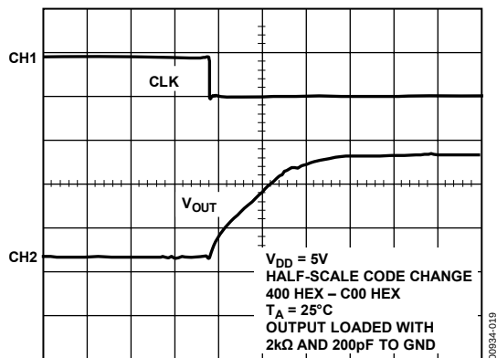
Figure 19. Half-Scale Settling Time
