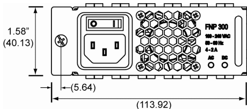
Figure 3 - Mechanical Dimension
