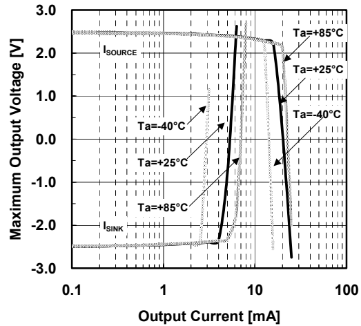
Output Voltage vs. Output Current (correlation with T_a )
