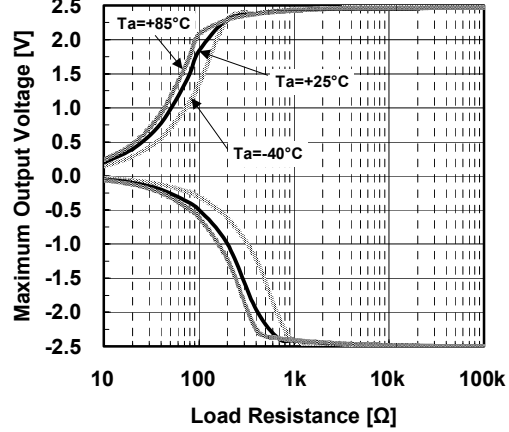
Maximum Output Voltage vs. Load Resistance (correlation with T_a )
