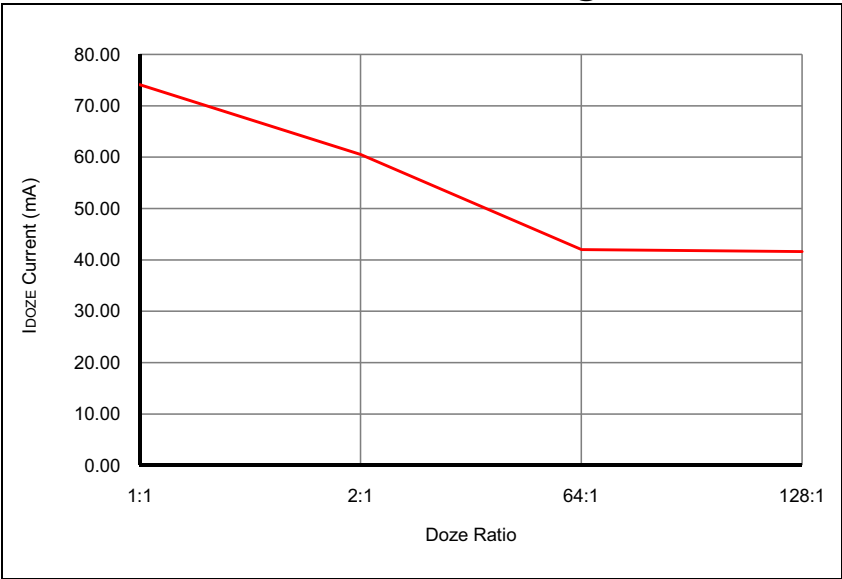
FIGURE 32-11: TYPICAL I_{DOZE} CURRENT @ V_{DD} = 3.3V , +85^{\circ}C
