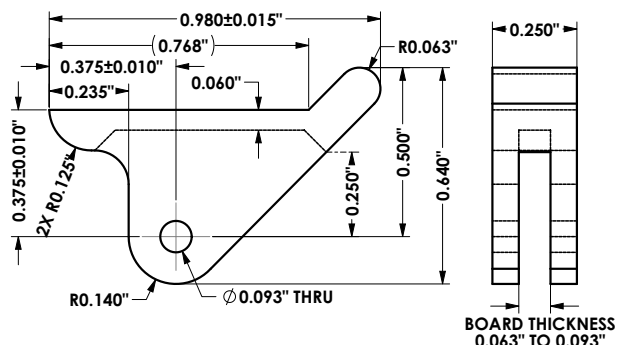
Rotation Type Ejector Handle - HA9
