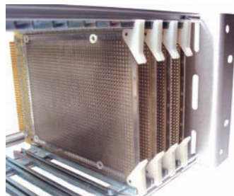
Rotation Type Ejector Handle - HA9
