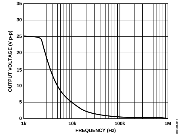
Figure 11. Large Signal Frequency Response
