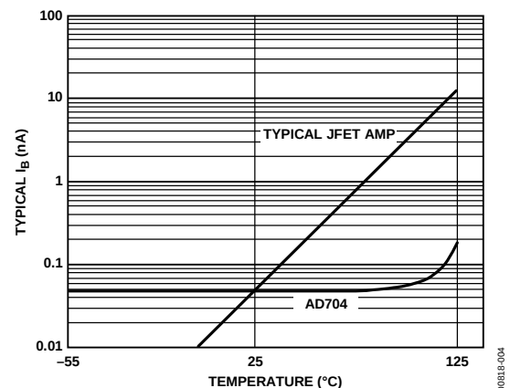
Figure 4. Input Bias Current Over Temperature
