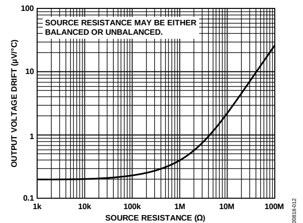
Figure 12. Offset Voltage Drift vs. Source Resistance
