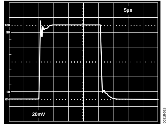
Figure 28. Unity Gain Follower Small Signal Pulse Response R_F = 0 \Omega , C_L = 100 pF
