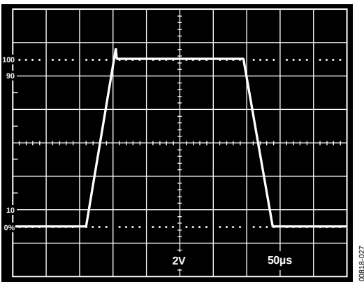
Figure 27. Unity Gain Follower Large Signal Pulse Response R_F = 10 k\Omega , C_L = 1000 pF
