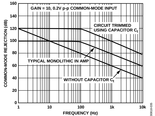
Figure 35. Common-Mode Rejection vs. Frequency with and Without Capacitor C_t
