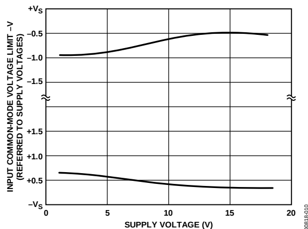
Figure 10. Input Common-Mode Voltage Range vs. Supply Voltage
