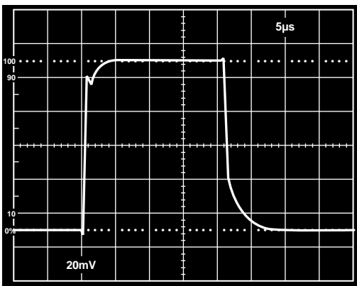
Figure 32. Unity Gain Inverter Small Signal Pulse Response, C_L = 100 \text{ pF}
