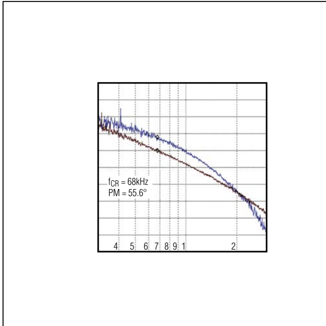
Figure 3. MAX17502G Full-Load Bode Plot ( V_{IN} = 24\text{V} )
