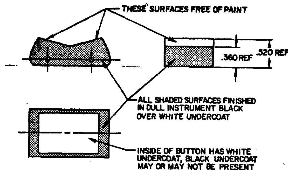
DETAIL A
