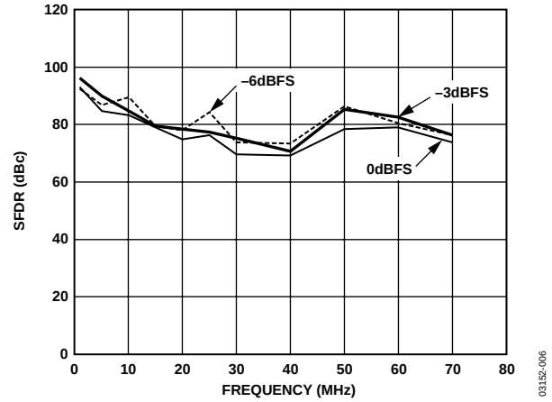
Figure 6. SFDR vs. Frequency, f_{DATA} = 200 MSPS, 2x Interpolation
