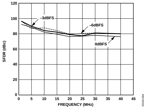
Figure 4. SFDR vs. Frequency, f_{DATA} = 100 MSPS, 4x Interpolation
