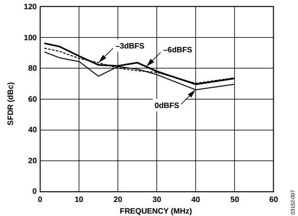
Figure 7. SFDR vs. Frequency, f_{DATA} = 125 MSPS, 4x Interpolation
