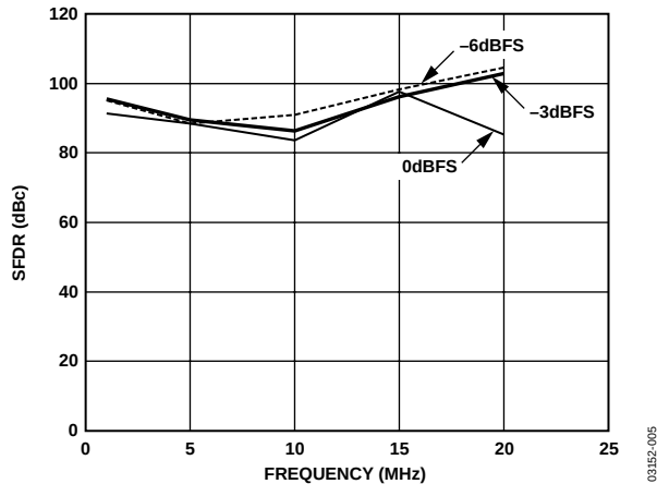
Figure 5. SFDR vs. Frequency, f_{DATA} = 50 MSPS, 8x Interpolation
