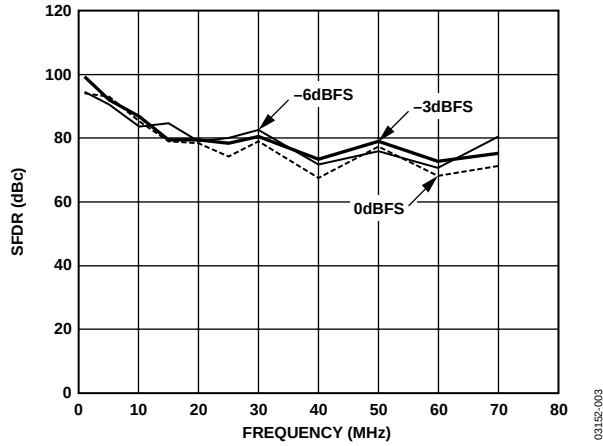
Figure 3. SFDR vs. Frequency, f_{DATA} = 200 MSPS, 1x Interpolation
