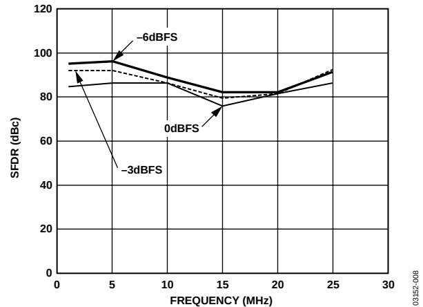
Figure 8. SFDR vs. Frequency, f_{DATA} = 62.5 MSPS, 8x Interpolation
