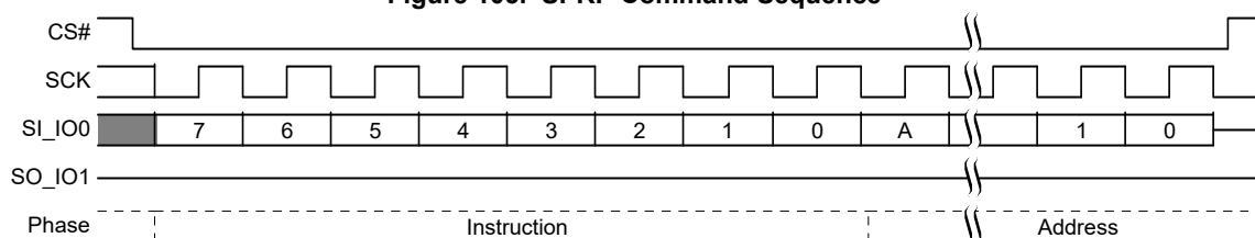
Figure 105. SPRP Command Sequence
