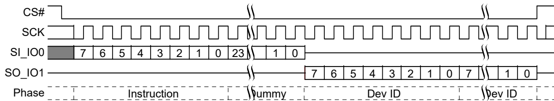
Figure 127. Read Identification (RES) Command Sequence
