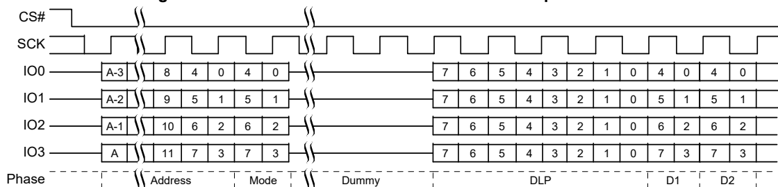
Figure 76. Continuous DDR Quad I/O Read Subsequent Access
